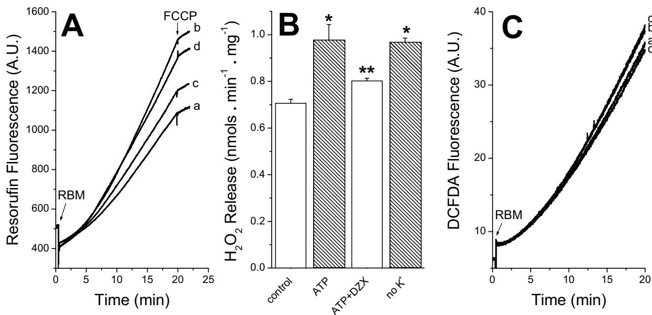
Fig. 1. K + transport through mitoK ATP decreases ROS release in brain mitochondria. Rat brain mitochondria (RBM, 0.2 mg/ml) were added to reaction media at 37°C containing 150 mM KCl, 10 mM HEPES, 2 mM Mg 2+ , 1 mM EGTA, 1 mM P i , 2 mM malate, 2 mM glutamate, 1 mg/ml BSA, 2 μg/ml oligomycin, pH 7.2 (KOH). Amplex Red (50 μM) and 1 U/ml HRP (panels A and B) or 10 μM H_2DCFDA (panel C) were present to measure ROS production under control conditions (no further additions, lines a) or in the presence of 1 mM ATP (lines b), 1 mM ATP and 10 μM DZX (lines c), or no further additions, in a media in which all K + salts were substituted for Na + (lines d). FCCP (2 μM) was added where indicated. Panel B represents average \pm S.E.M. H_2O_2 release rates, observed between 10 and 20 min after mitochondrial addition using three different mitochondrial preparations. * P < 0.05 compared to control, ** P < 0.05 compared to the experiment conducted in the presence of ATP.
